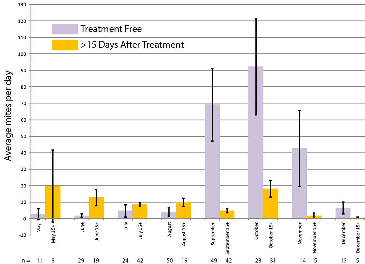
FIGURE 6 – Comparison of Treatment Free and Treated colonies (using only mite counts after 15 days past treatment) by month; with the 95% confidence intervals.
