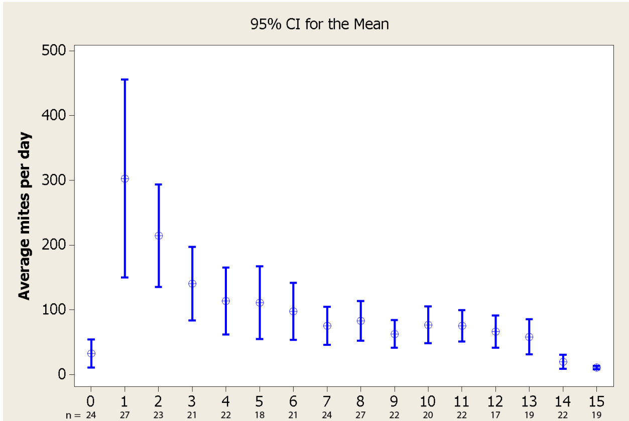
FIGURE 5 – Immediate effect of treatments (MAQs, ½ MAQs, and Hopyguard together) based upon the day treated (Time 0) and the resulting 15 days after; with the 95% confidence intervals.
